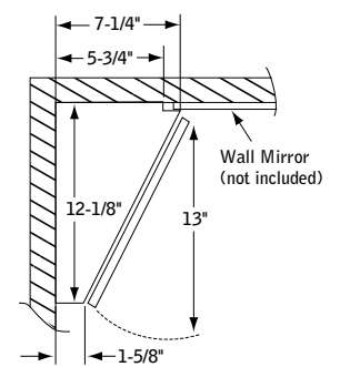
Top-down view of left hand Avanti 631 Corner Cabinet as shown in photo above.
