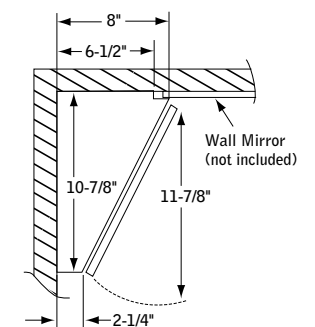
Top-down view of left hand Avanti 637 Corner Cabinet.
